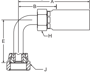
58/58H Series Permanent (SAE Drop Dimensions)
