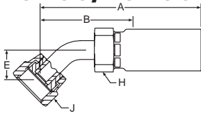
58/58H Series Permanent (SAE Drop Dimensions)
